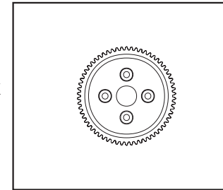
PD2125 SPUR GEAR/ 67T, ZK
