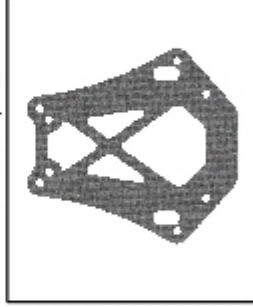
PD8225 CFRP FRONT SHOCK TOWER
